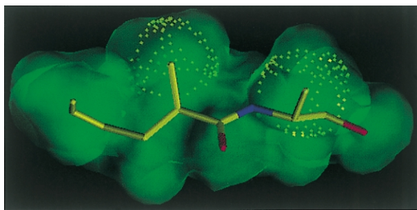
Figure 2. CB1 receptor excluded volume map as calculated by adding the molecular volumes of the aligned 'active' analogues ( 1 , 2 , 4 , 13 , and 15 ). The yellow colored clouds represent the volumes occupied by the methyl groups of the most active analogue, 4 .
