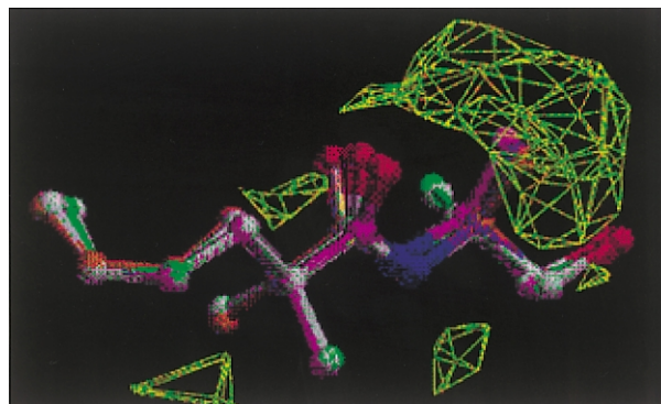
Figure 1. CB1 receptor essential volume map as calculated by subtracting the sum of molecular volumes of the aligned 'inactive' analogues ( 5 , 6 , 7 , and 14 ), from the sum of molecular volumes of the aligned 'active' ones ( 1 , 2 , 4 , 13 , and 15 ). By extrapolation, the yellow contours correspond to areas occupied by structural features of the receptor.
