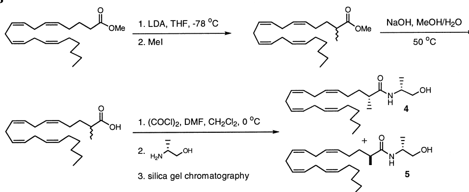
Scheme 1. Synthesis of chiral methylated anandamide analogues.
